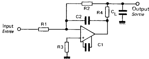
ISOLATING LARGE CAPACITIVE LOADS ISOLEMENT DES CHARGES TRES CAPACITIVES
